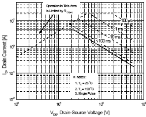
Figure 9-1. Maximum Safe Operating Area for OSP4N60C
