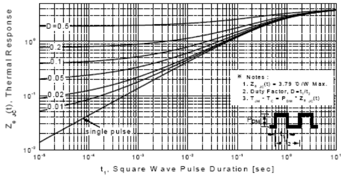
Figure 11-2. Transient Thermal Response Curve for OSF4N60C
