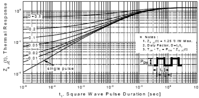
Figure 11-1. Transient Thermal Response Curve for OSP4N60C
